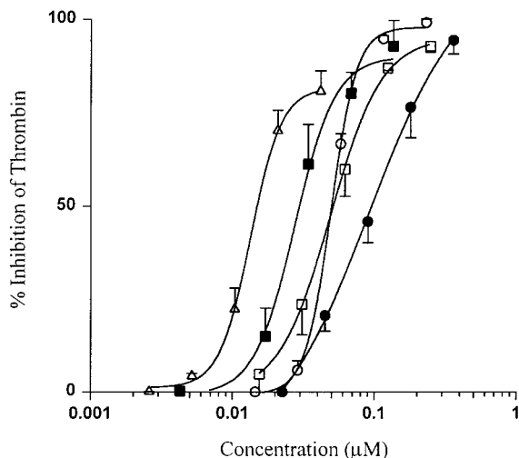
Figure 2. Effect of 1 (○), 2 (●), 4 (Δ), 6 (□), and 7 (■) on the inhibitory activity of thrombin-induced fibrin-clotting. Points shown are means of triplicate \pm standard derivation.
